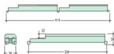
Module Driver Dimensions
