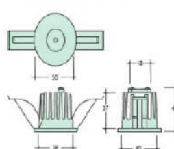
Lamphead Dimensions
